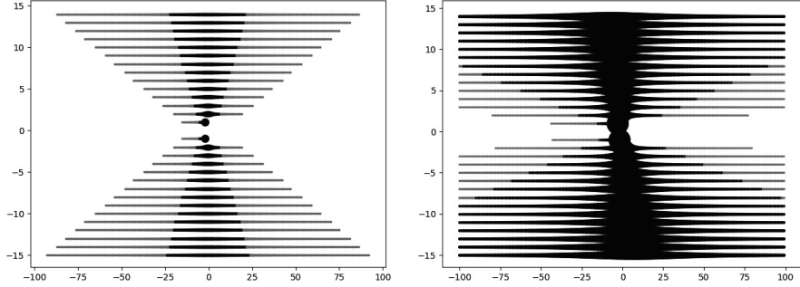
Figure 1: The x axis represents a , the y axis represents the b values. The points represent the values \frac{\gamma}{1-r_m} for F = 2 (left) and F = 7 (right) in the neighbourhood of the origin. Darker points represent higher values.
