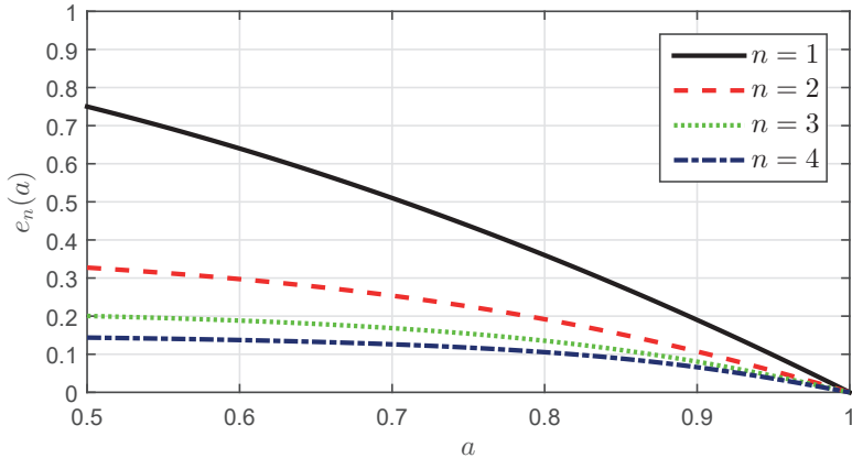
Figure 1. The tolerated error rate depending on the absolute value of the inverse pole, for n = 1, 2, 3, 4 .
