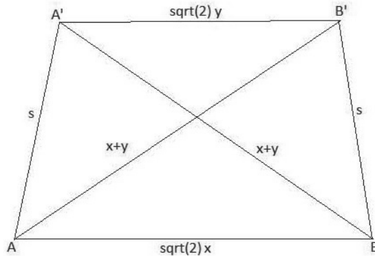
Figure 3.2. Isosceles trapezoid: one of the 4 congruent faces of the TSP.
