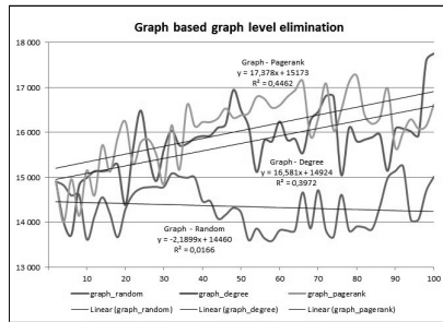
Figure 1. Graph-level elimination in AMAZON PRODUCT CO-PURCHASING NETWORK
