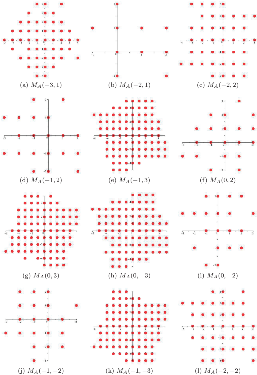
Figure 1: Digit sets of simultaneous Gaussian number systems
