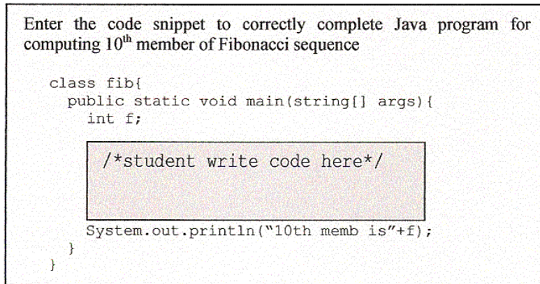
Figure 9. Skeleton program
