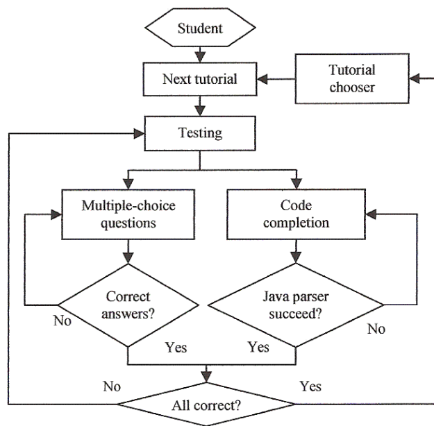
Figure 5. Flow chart of Mag module for testing of student's knowledge
