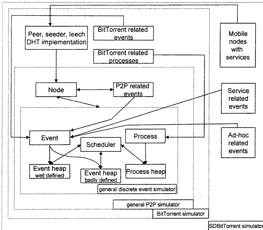
Figure 1. Simulator components
