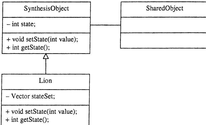
Figure 3. Class diagram of the example
