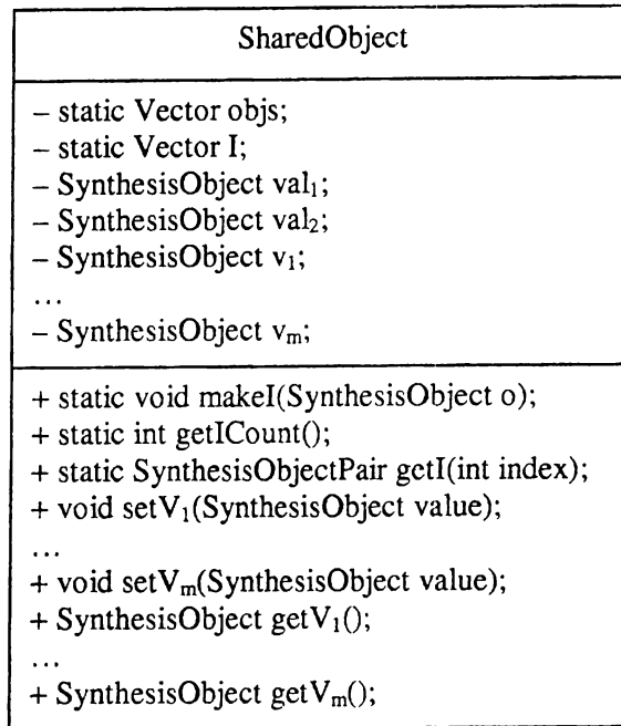
Figure 2. Class SharedObject
